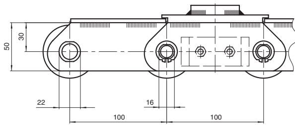
Chain P. 100x30x55 øR
